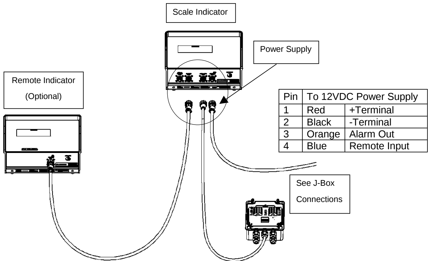
Indicator Connection Diagram
