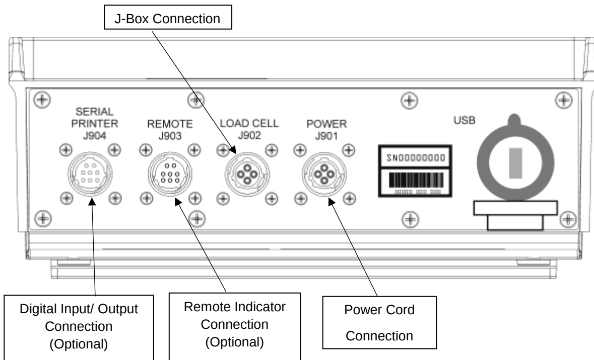
Indicator Connection Diagram
